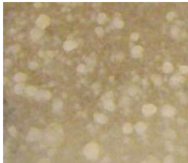
Figure 1: Colony Morphology
