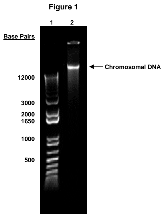
Lane 1: Invitrogen™ TrackIt 1 Kb Plus DNA Ladder™ Lane 2: 200 ng of HM-122D
